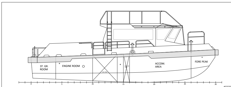
Profile View
