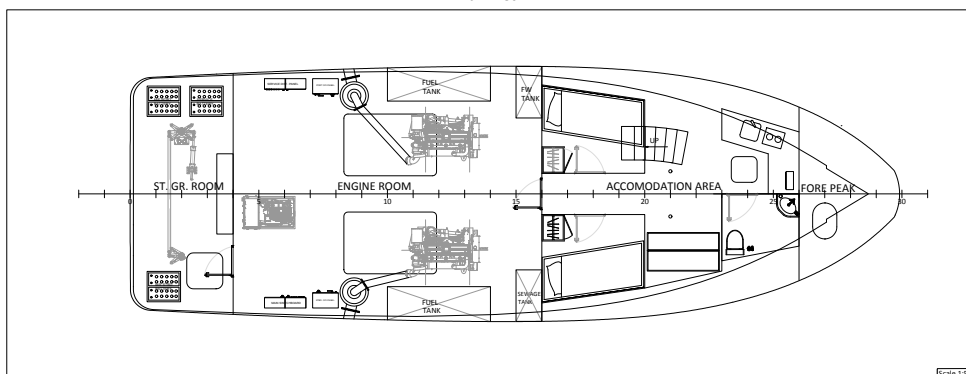
Lower Deck
