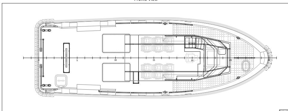
Main Deck
