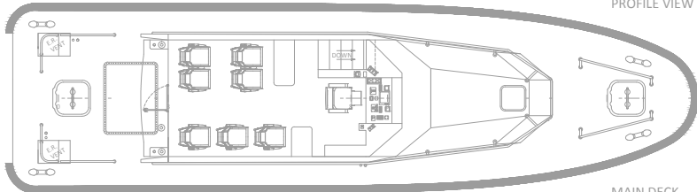
MAIN DECK
