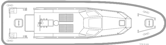
TOP PLAN
