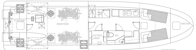
LOWER DECK
