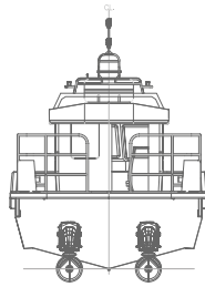
AFT VIEW
