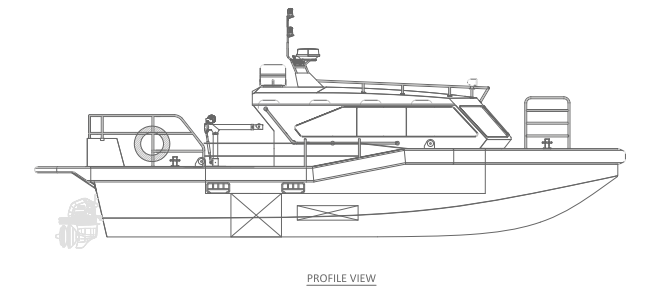
PROFILE VIEW
