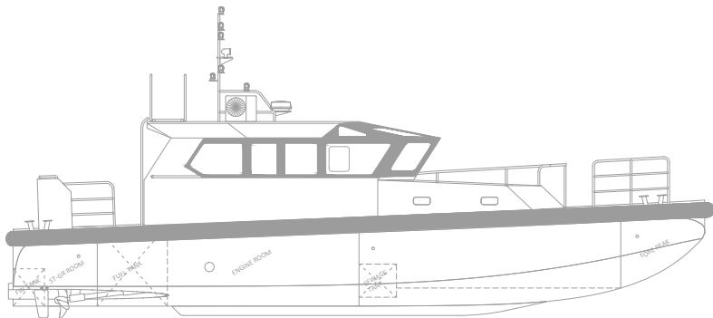
PROFILE VIEW
