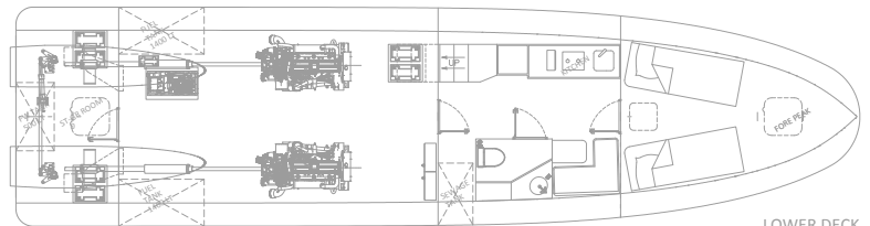
LOWER DECK
