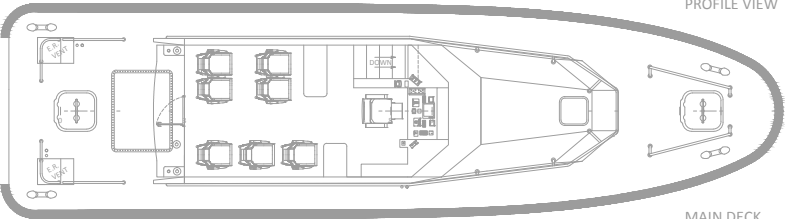
MAIN DECK
