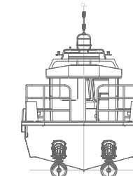
AFT VIEW
