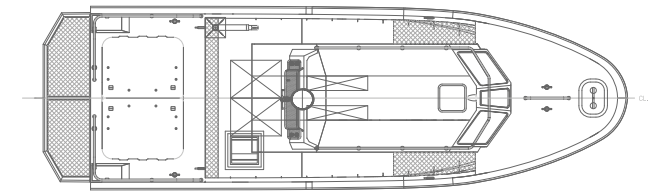
PLAN VIEW
