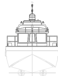
FWD VIEW
