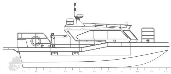
PROFILE VIEW
