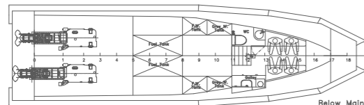
Below Maindeck
